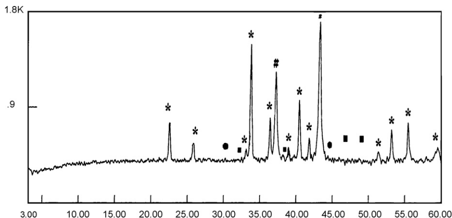
Fig. 7. XRD of NiB annealed to 1073 K. *, phase of \text{Ni}_3(\text{BO}_3)_2 (JCPDS 261284); #, phase of NiO (JCPDS 40835); ●, phase of NiB (JCPDS 60567); ■, phase of Ni (JCPDS 40850).
