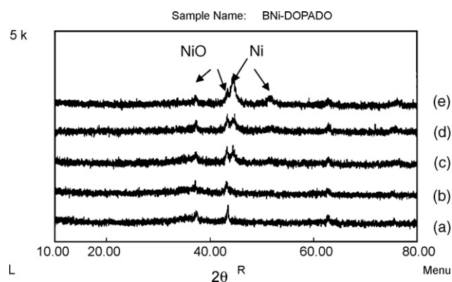
Fig. 9. XRD of nickel metallic dopants borides: (a) ZnNiB, (b) MnNiB, (c) NiB, (d) CoNiB, and (e) CrNiB.
